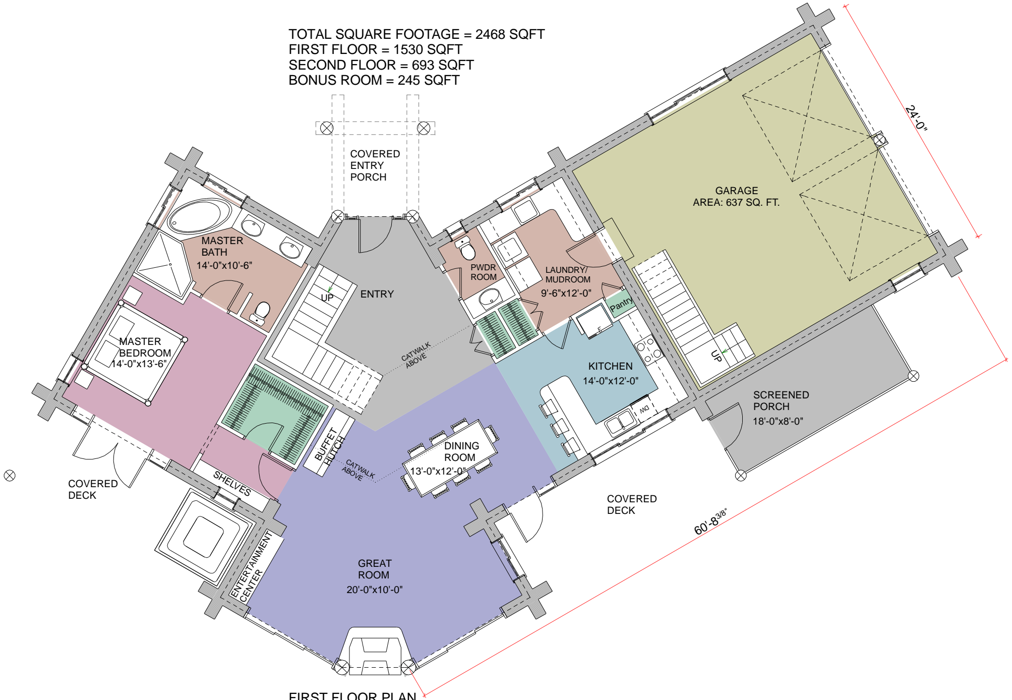
FIRST FLOOR PLAN AREA=1530 SQFT
