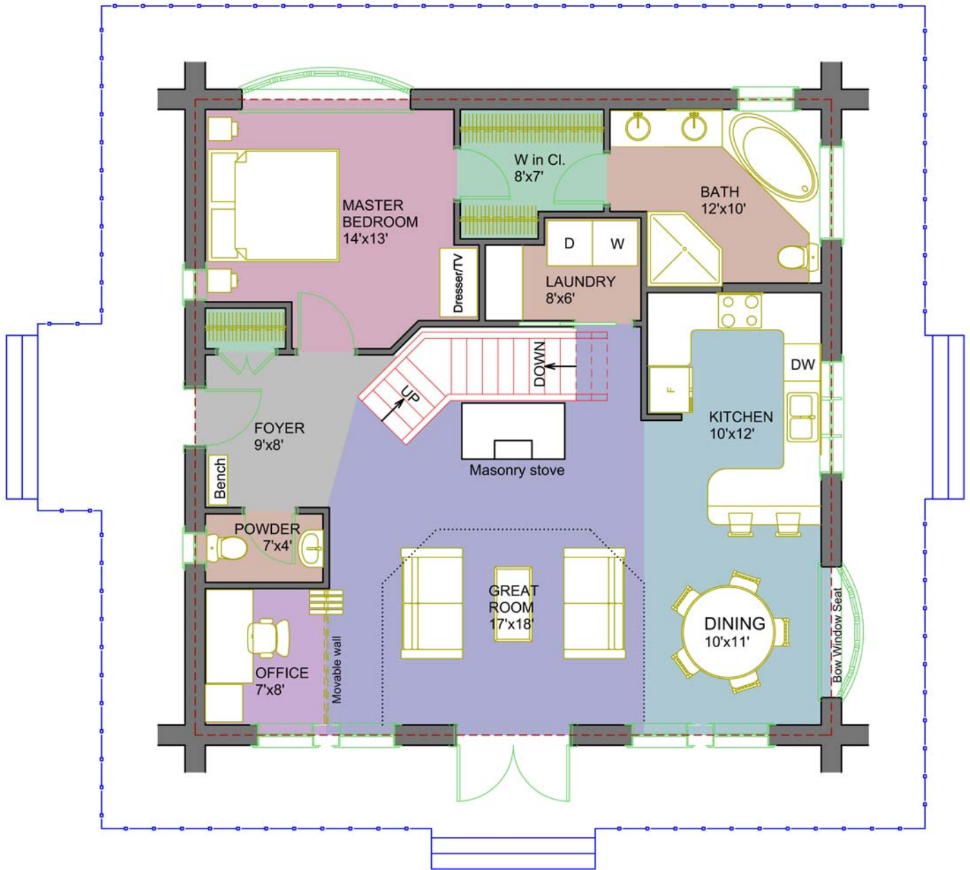
FIRST FLOOR PLAN AREA: 1190 SQ.FT.
