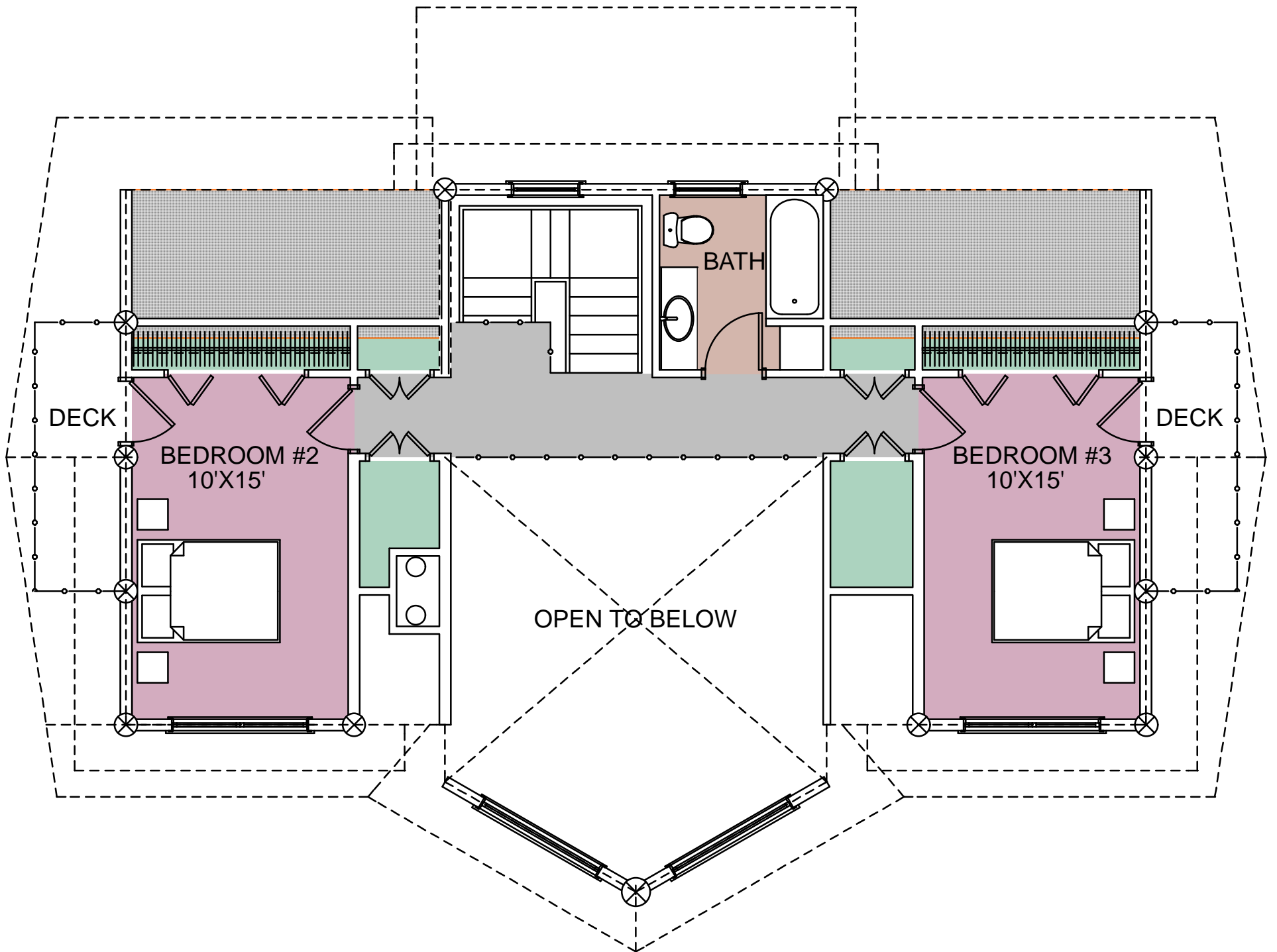
SECOND FLOOR PLAN AREA: 550SQ. FT.
