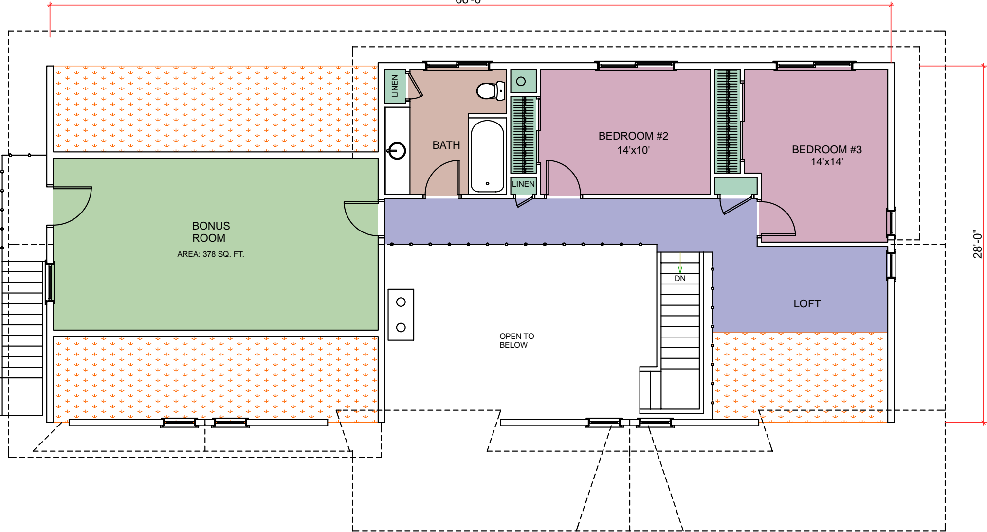
SECOND FLOOR PLAN AREA: 678 SQ. FT.
