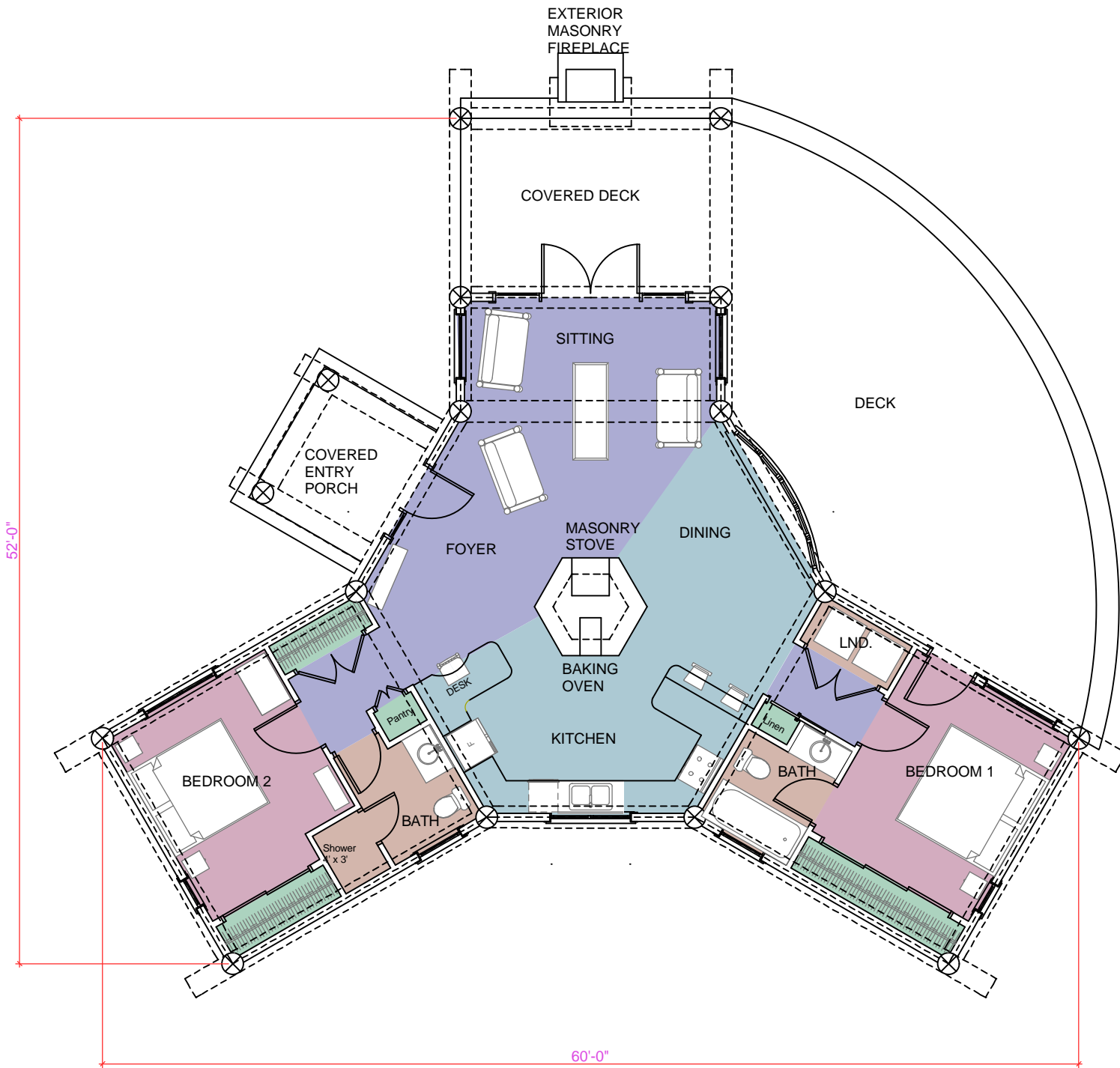
FIRST FLOOR PLAN AREA: 1267 SQ.FT.
