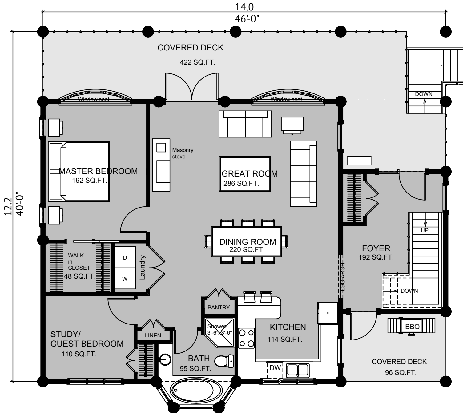
FIRST FLOOR PLAN AREA: 1302 SQ. FT./ 121 SQ.M
