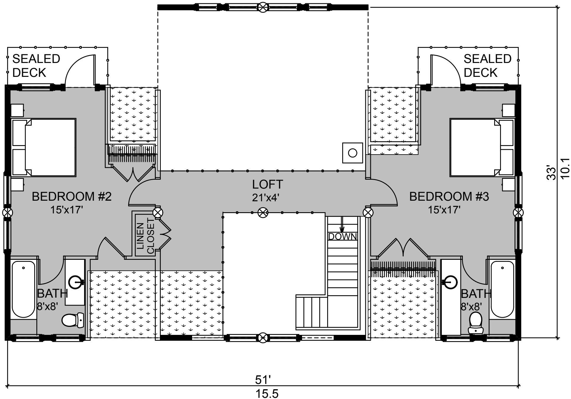
SECOND FLOOR PLAN AREA: 747 SQ. FT. 69.40 SQ.M.
