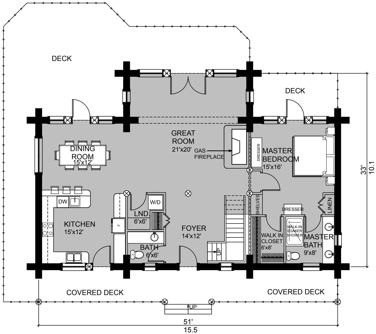
FIRST FLOOR PLAN AREA: 1485 SQ.FT. 137.96 SQ.M.
