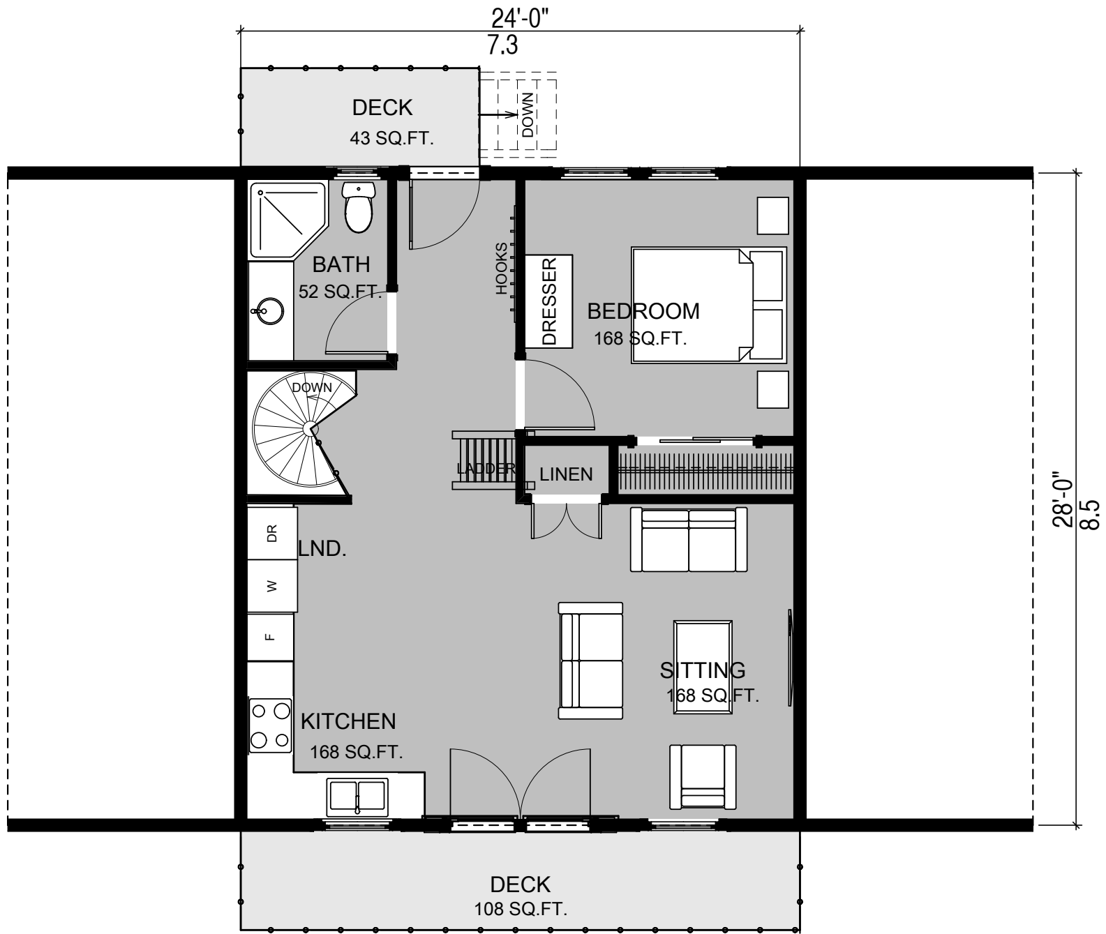
SECOND FLOOR PLAN AREA: 561 SQ. FT. 52 SQ.M.
