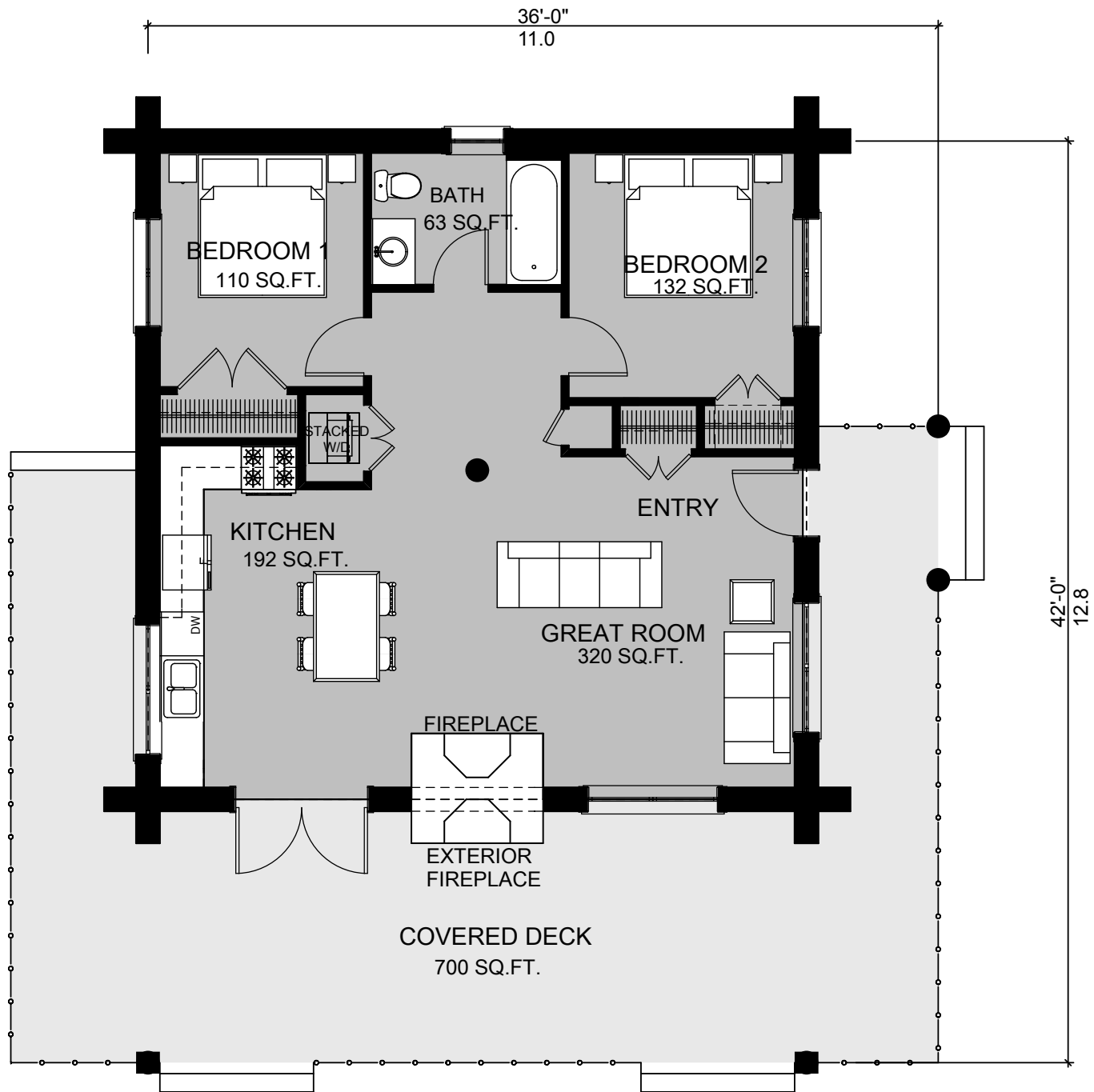
FIRST FLOOR PLAN AREA: 930 SQ. FT. 83 SQ.M.
