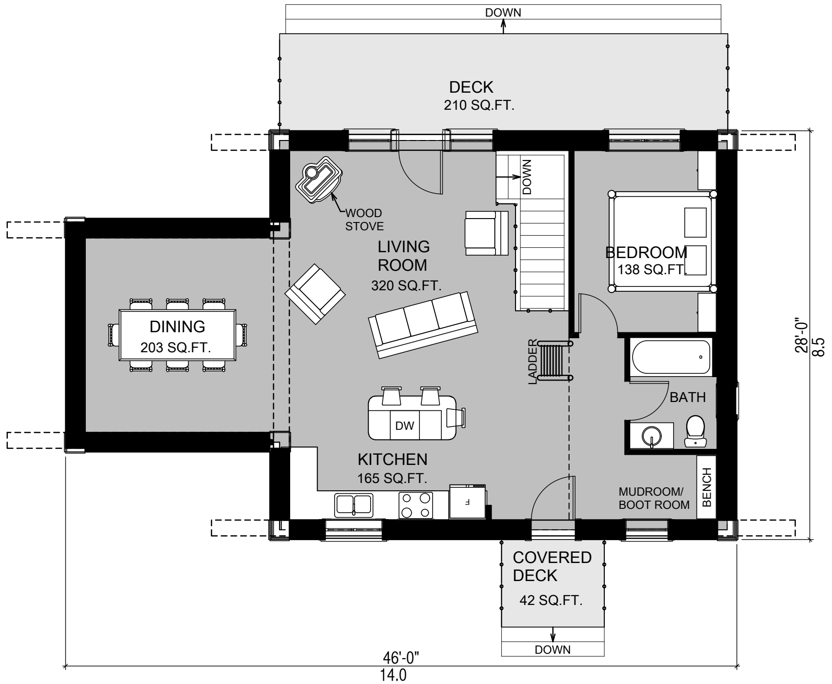
FIRST FLOOR PLAN AREA: 1071 SQ.FT. / 99.5 SQ. M
