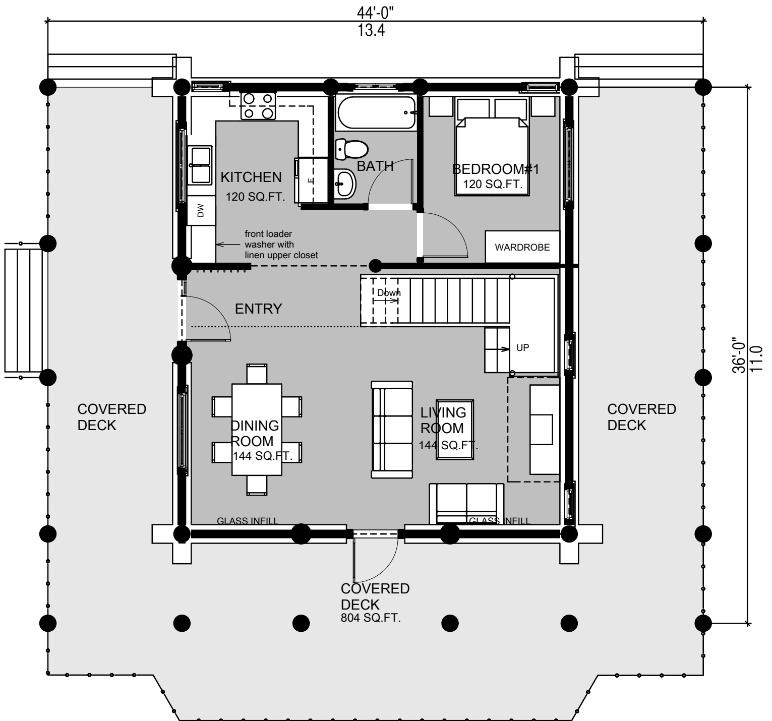
FIRST FLOOR PLAN AREA: 780 SQ.FT. 72.46 SQ.M.
