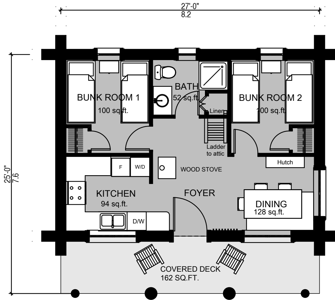
FIRST FLOOR PLAN AREA: 513 SQ.FT. / 47.7 SQ.M
