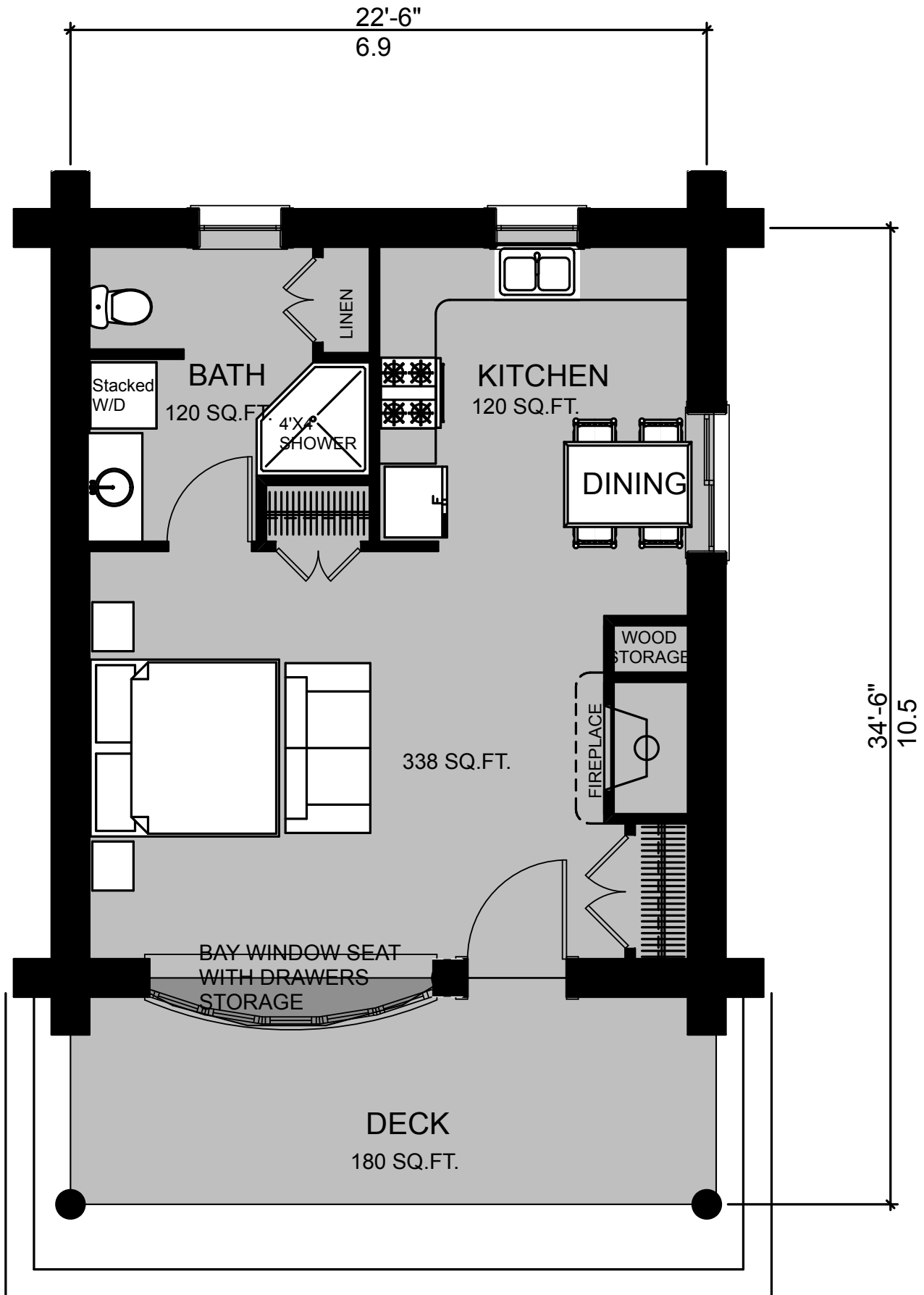
FIRST FLOOR PLAN AREA: 600 SQ.FT./ 56 SQ.M.
