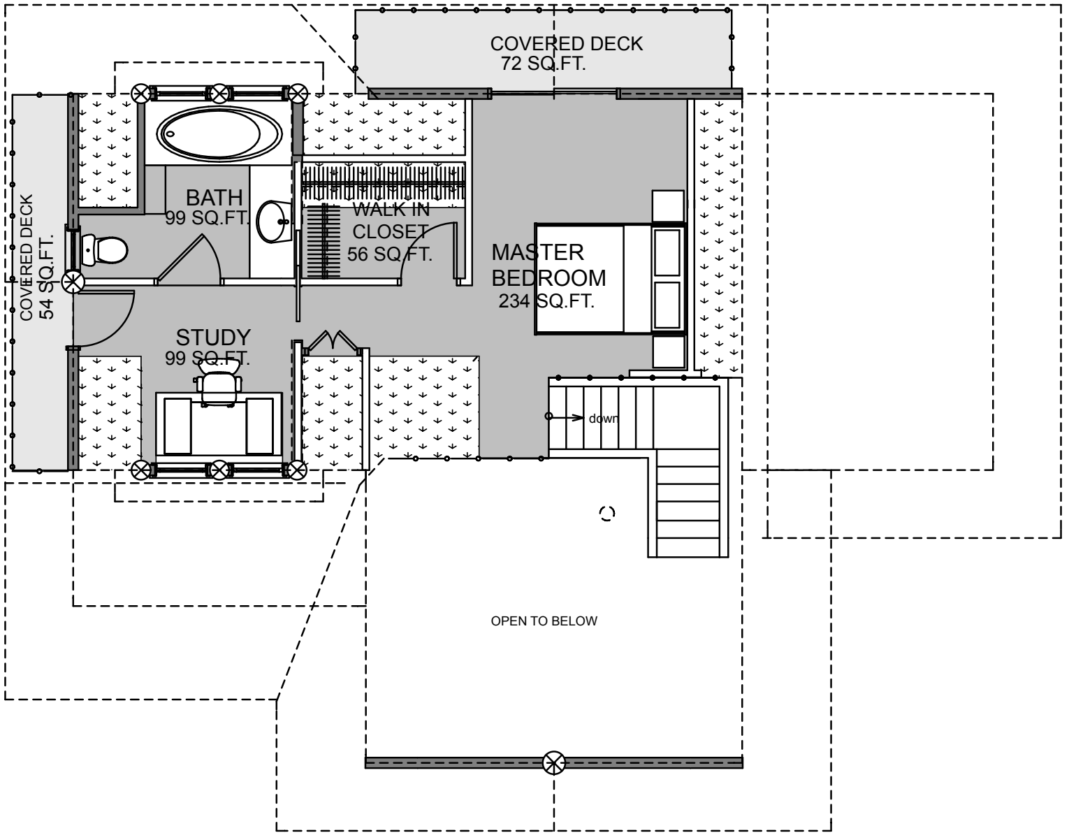
SECOND FLOOR PLAN AREA: 360 SQ. FT. 33.45 SQ.M.
