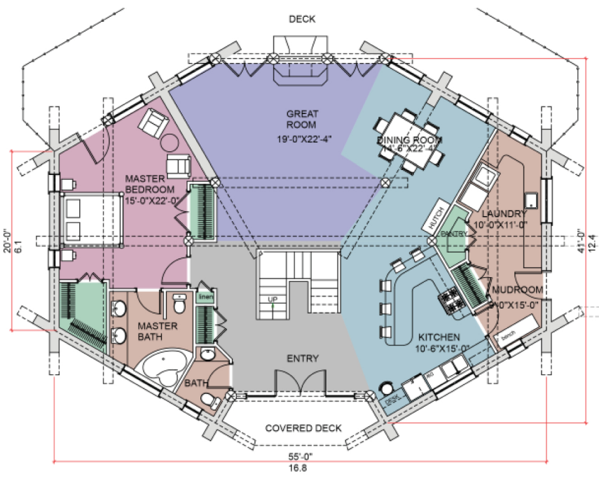
FIRST FLOOR PLAN AREA: 1858 SQ. FT. 172.6 SQ.M.
