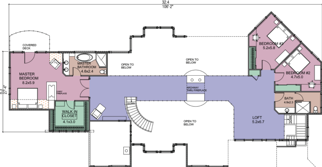
SECOND FLOOR PLAN AREA: 1197 SQ.FT. 185.8 SQ. M
