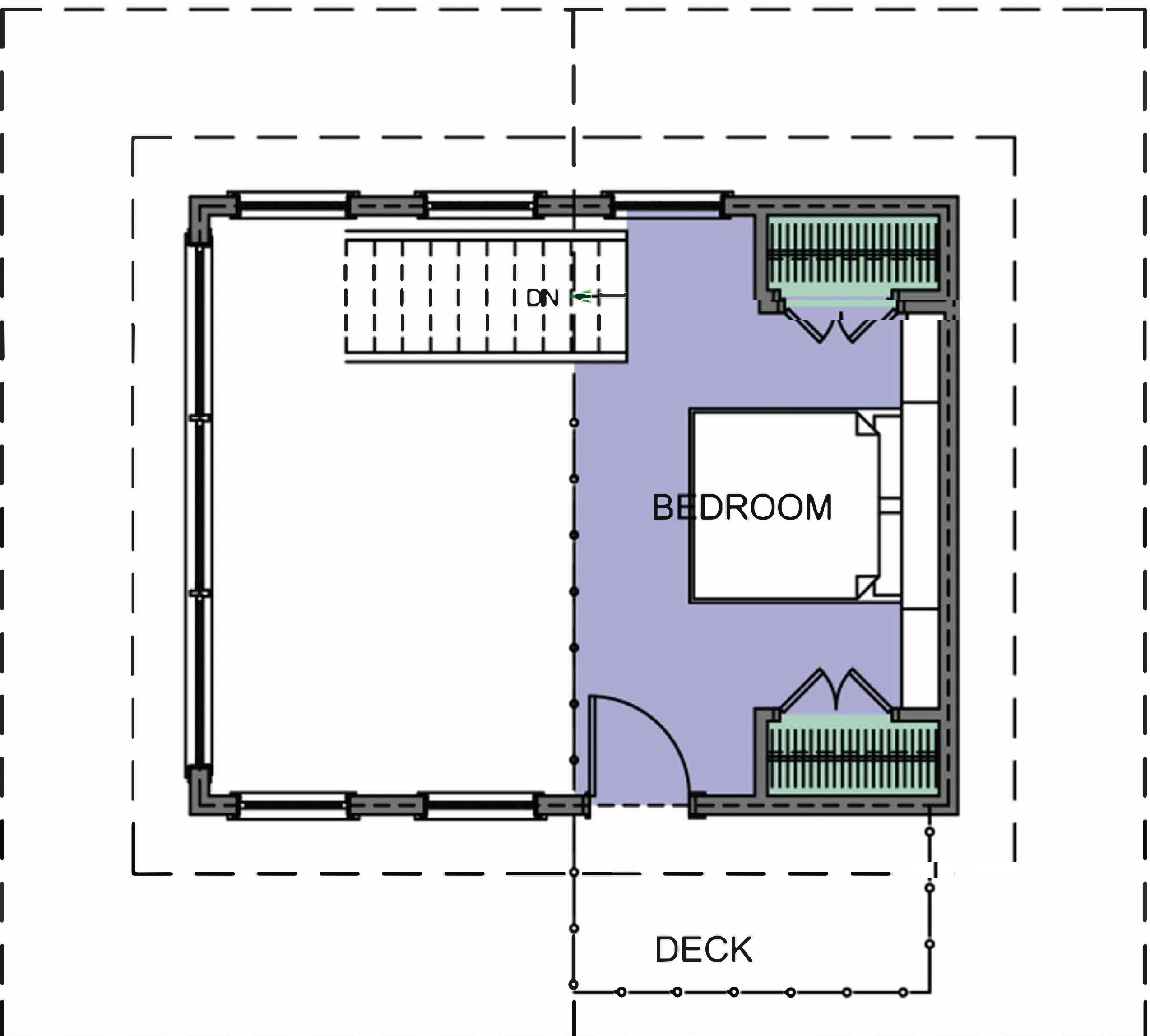
SECOND FLOOR PLAN AREA: 150 SQ. FT. / 13.9 SQ. M
